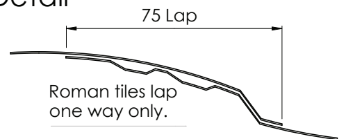
Figure 3.4 Lap Section
