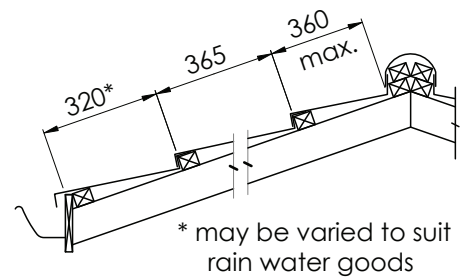
Figure 3.5 Batten Layout
