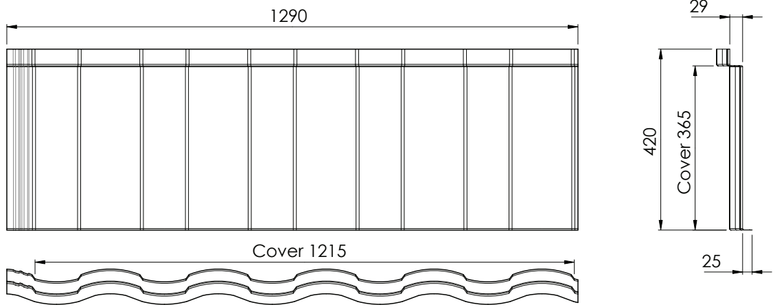
Figure 3.1 Tile Dimensions
